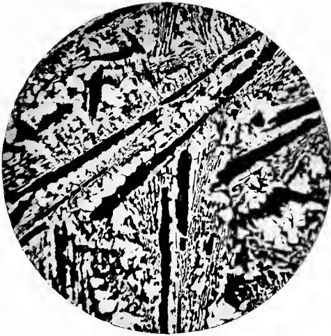
A. Antimony 75, copper 25%. \times 86 .
